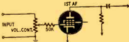
Fig. 3—Grid resistor eliminates instability.
