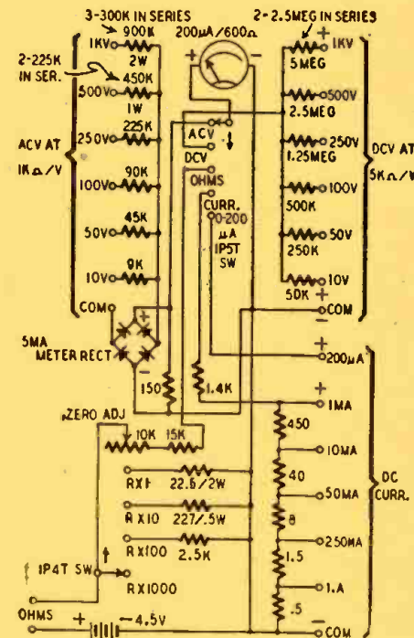
Multimeter with a 200-microampere movement.
