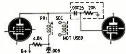
Fig. 3—Coupling inductance in plate circuit. (The secondary is not used for the discriminator signal frequency). The oscillator is tracked at the low-frequency end by adjusting C s , and at the high-frequency end by adjusting C p . The coil can be squeezed together or spread apart as required. Alignment is checked by varying the inductance of each coil with a tuning wand. The powdered-iron slug low-
