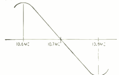
Fig. 2—A good discriminator curve is linear.
