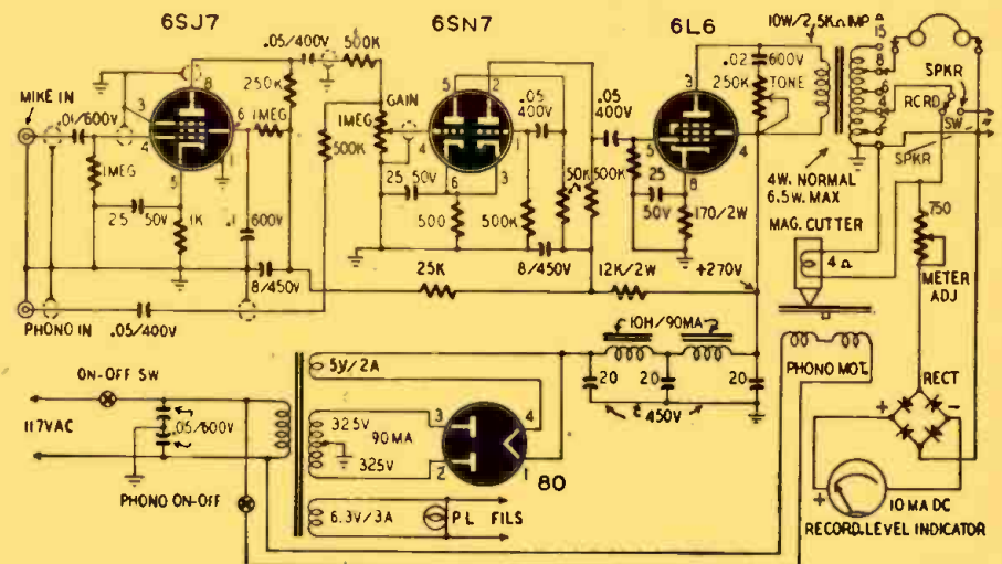
This medium-power recording amplifier uses a 10-milliamperere meter as level indicator.
